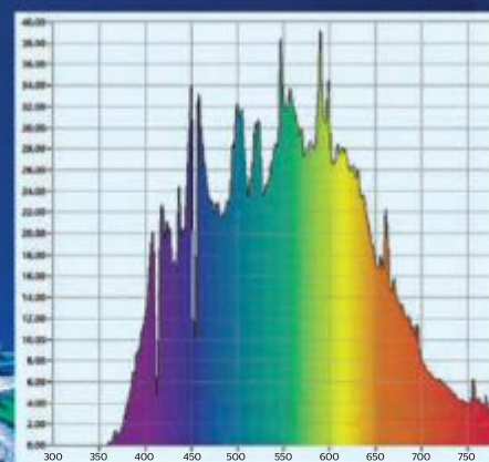
Chameleon's Plasma Lamp
